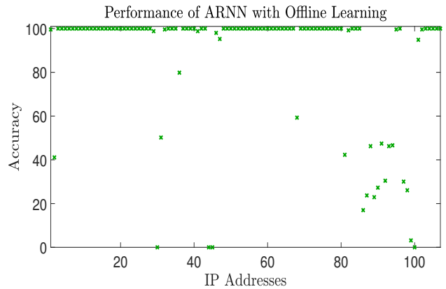
FIGURE 2: The average accuracy of the ARNN predictions for all addresses 1 \leq i \leq 107 is shown for the test data TD , by comparing the ground truth binary value Y_i^l with the ARNN's binary output Z_i^l .
