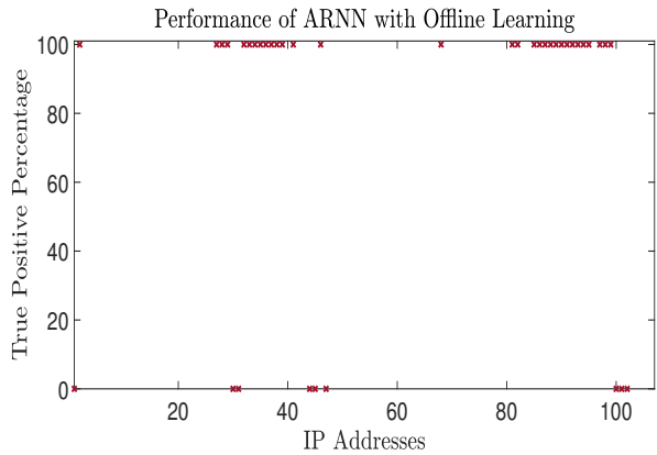
FIGURE 3: The average percentage TPR is shown over all the slots for each of the 107 addresses in the network, obtained by comparing Y_i^l and Z_i^l for those values of l where Y_i^l = 1 . Note that if Y_i^l = 0 for an address i in all the slots l in the TD , then the TPR cannot be measured for i . Thus only 39 out of 107 addresses are concerned by the TPR, as shown in the figure.
