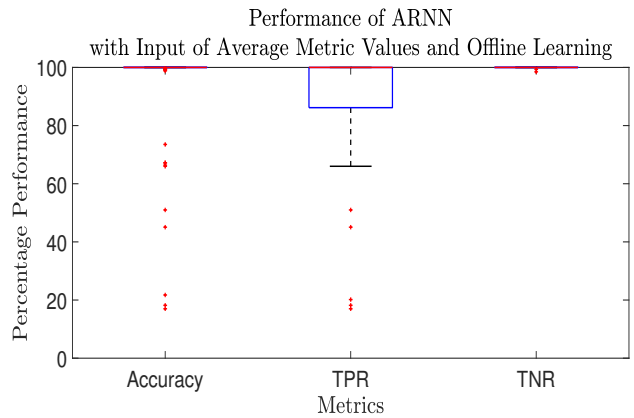
FIGURE 7: The Accuracy, TPR, TNR of the ARNN algorithm are shown as box-plots for the ARNN trained and tested with the Average Metric values for 458 \leq l \leq 713 .
